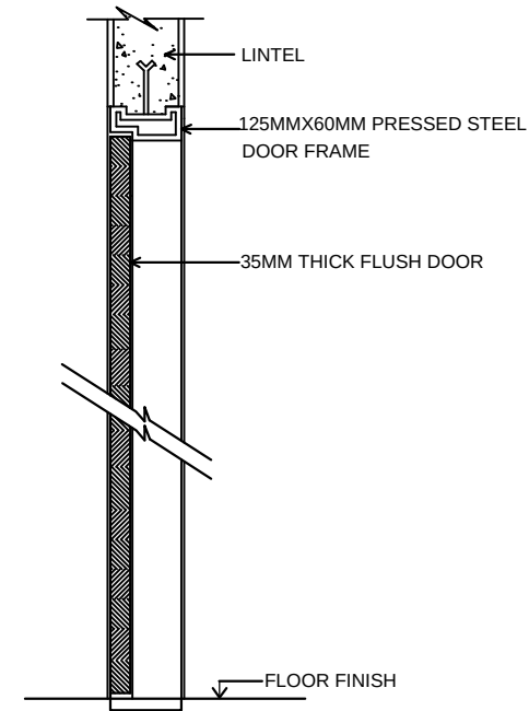
SECTION YY
