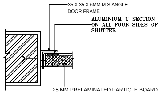
DETAIL AT A
