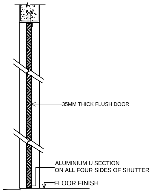
SECTION AT Y'-Y'
